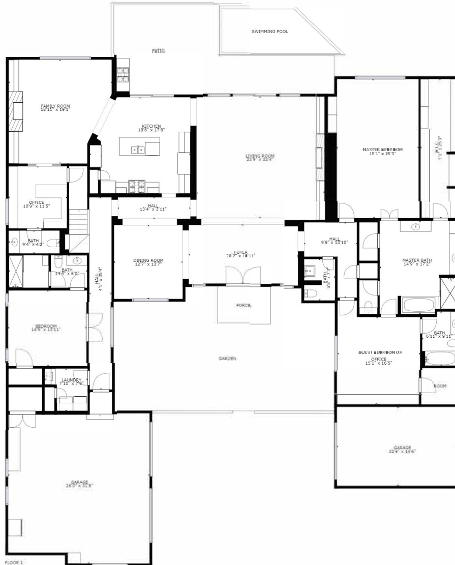
FLOOR 1 Floor 1
